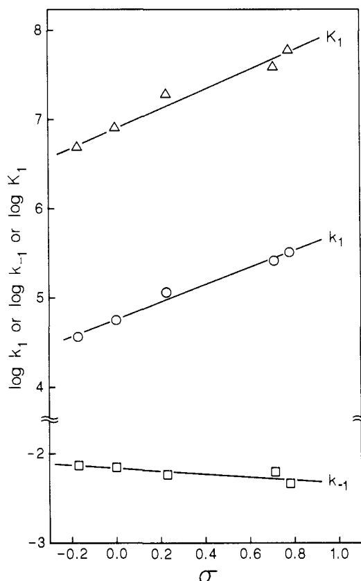
Figure 5. Hammett plots of k_1 , k_{-1} , and K_1 for the addition of HOC_2H_4S^- to substituted \alpha -nitrostilbenes.
