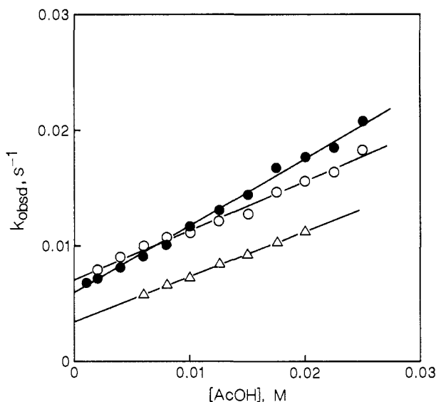
Figure 3. Representative plots of k_{obsd} vs [AcOH] in pH-jump experiments: \circ , HOCH_2CH_2S^-/4-CH_3 ; \bullet , HOCH_2CH_2S^-/4-Br ; \Delta , EtS^-/H .
