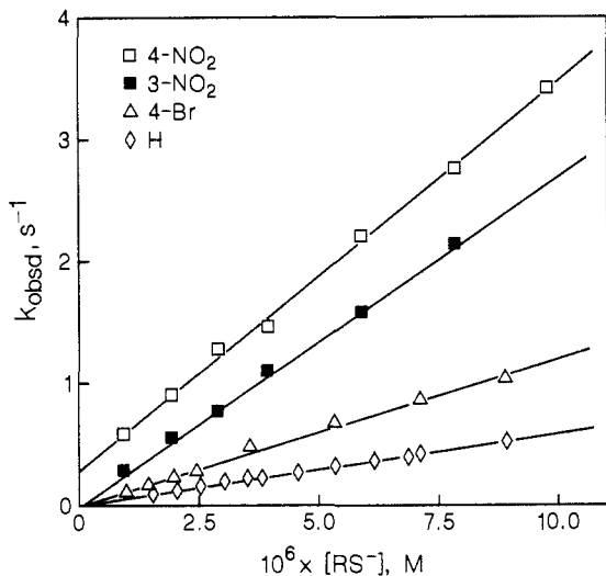
Figure 2. Representative plots of k_{obsd} vs [RS^-] for the reaction of substituted \alpha -nitrostilbenes with HOCH_2CH_2S^- .
